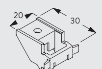
3603 Top fix bracket
