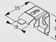
2302 Clip bracket
