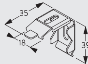
2302 Clip bracket
