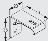
2343 Wall/Ceiling Bracket
