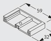
11174 Top Cover
