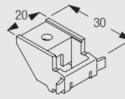
3603 Bracket (30mm)
