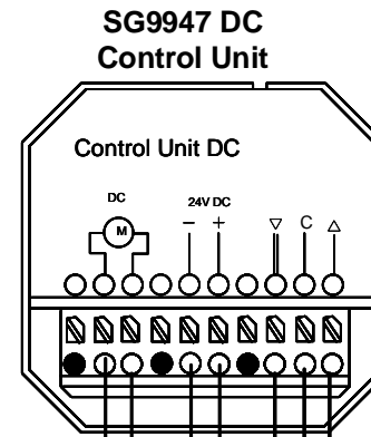
SG9947- Dimensions H 52mm x W49mm x D29mm
