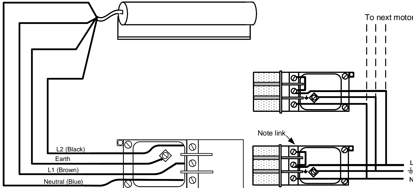
Plug set SG9916
